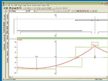
Reinforced concrete design to optimize bar layouts which can be passed into Bentley REBAR for detailing. Slabs can be linked to RAM Concept for RC and PT design.
